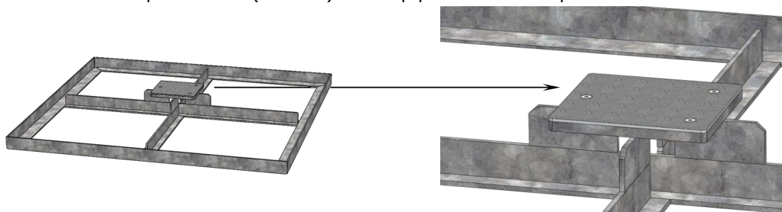
3-D views of lower part SZ010 (352535) with top plate for winter protection.
