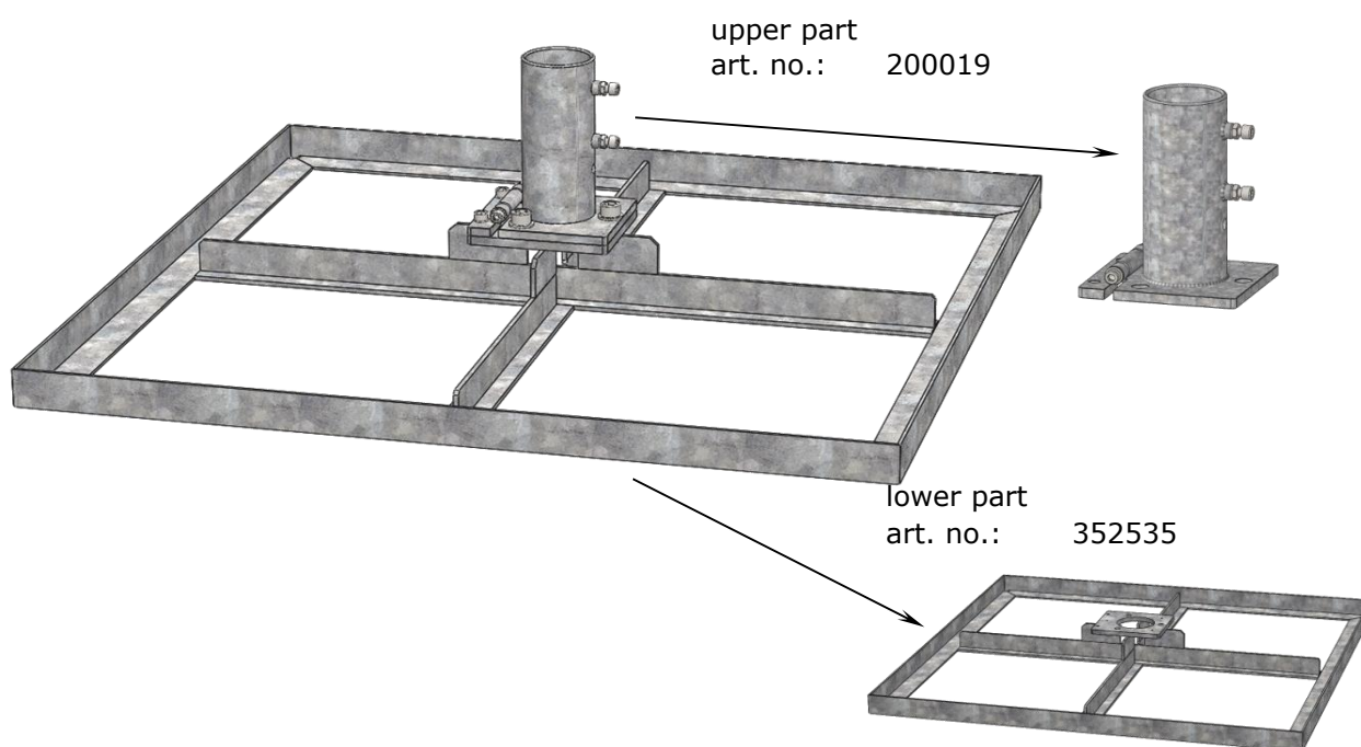
3-D views of SZ010
